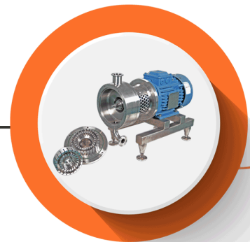
Homogenizer
