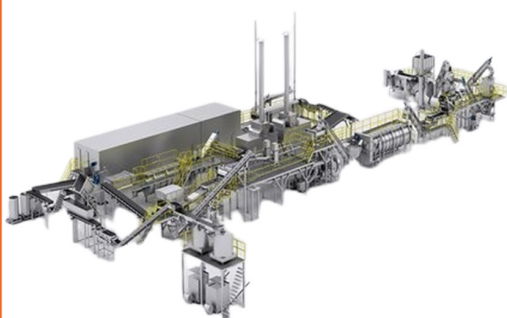
Mushroom & Vegetable Canning Processing Plant
